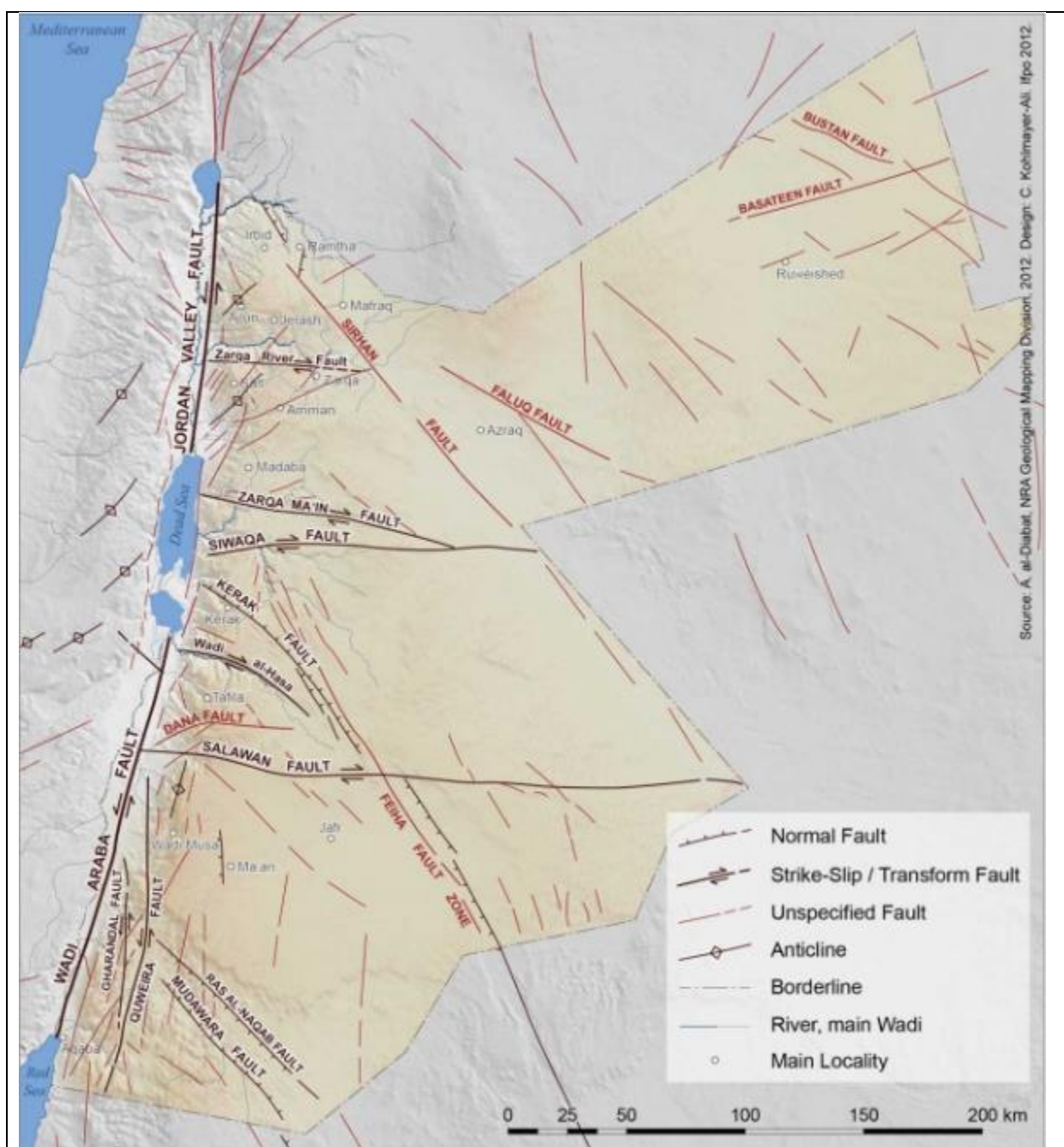
Jordan Major Structural Features 9
